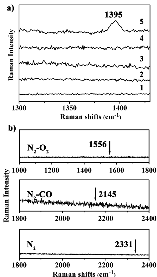
Figure 4. a) SERS spectra of single Au NPs (trace 1), single MOF-5 spheres (trace 2), and single core–shell Au@MOF-5 NPs with a shell thickness of (69.0 \pm 12.4) nm (trace 3), 25.1 \pm 4.1 nm (trace 4), and (3.2 \pm 0.5) nm (trace 5) toward \text{CO}_2 in the \text{CO}_2/\text{N}_2 gas mixture (the ratio is 1:5 for \text{CO}_2 vs. \text{N}_2 ) at room temperature. b) SERS spectra of single core–shell Au@MOF-5 NP with a shell thickness of (3.2 \pm 0.5) nm toward \text{N}_2 , \text{CO} , and \text{O}_2 . The arrows point to the characteristic SERS peak positions of \text{N}_2 , \text{CO} , and \text{O}_2 .
